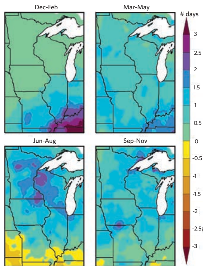
Figure 2. Modeled change in number of days/decade with >50 mm (2 in.) of precip. by season, 1961-2000 to 2045-2065
