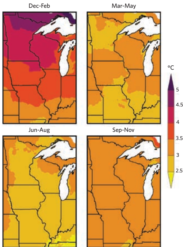
Figure 1. Modeled change in average temperature (°C) by season, 1961-2000 to 2045-2065
